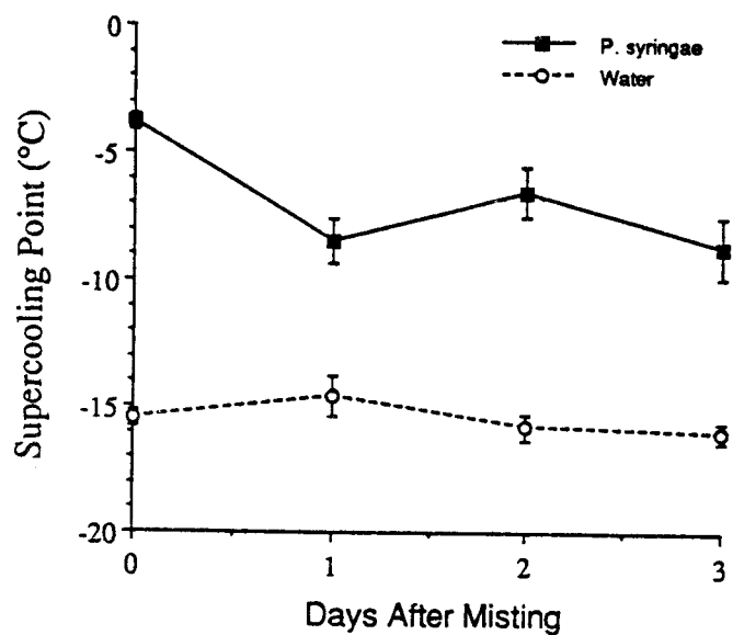
FIG. 2. Supercooling points of lady beetles ( H. convergens ) at the time of misting (day zero) and 1, 2, and 3 days after misting with water or P. syringae ( 10^8 bacteria per ml of water). The mouths of the insects were sealed to prevent ingestion. Supercooling points of P. syringae -treated individuals were significantly elevated above control values ( n = 10 to 12 ).
